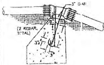
TYPE A RESTRAINT 11-1/4" & 22-1/2" VERTICAL OVER-BENDS
