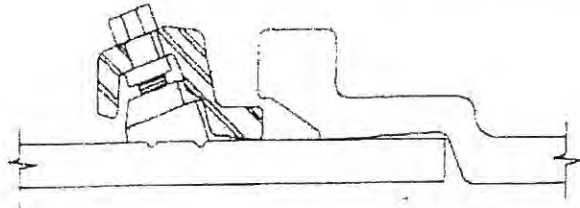
WEDGE DETAIL
