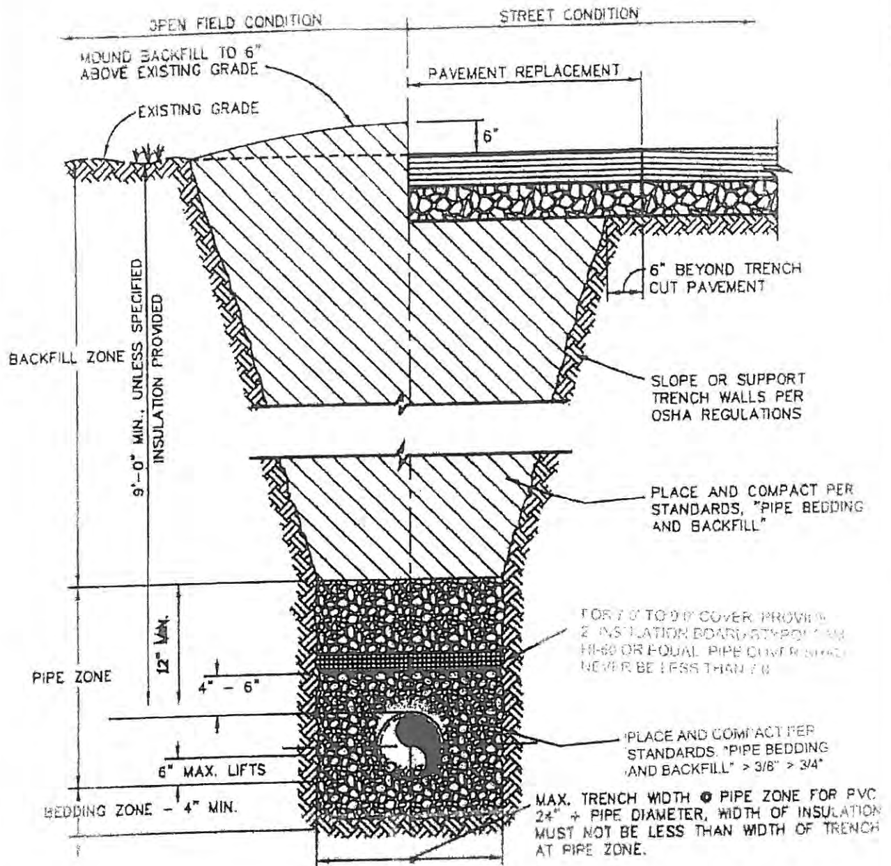
Water Main and Service Line Bedding and Backfill Detail
