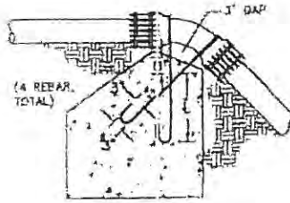
TYPE B RESTRAINT 45° VERTICAL UNDER-BENDS
